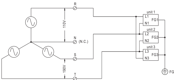
3 phase 4 line 190/110VAC system
